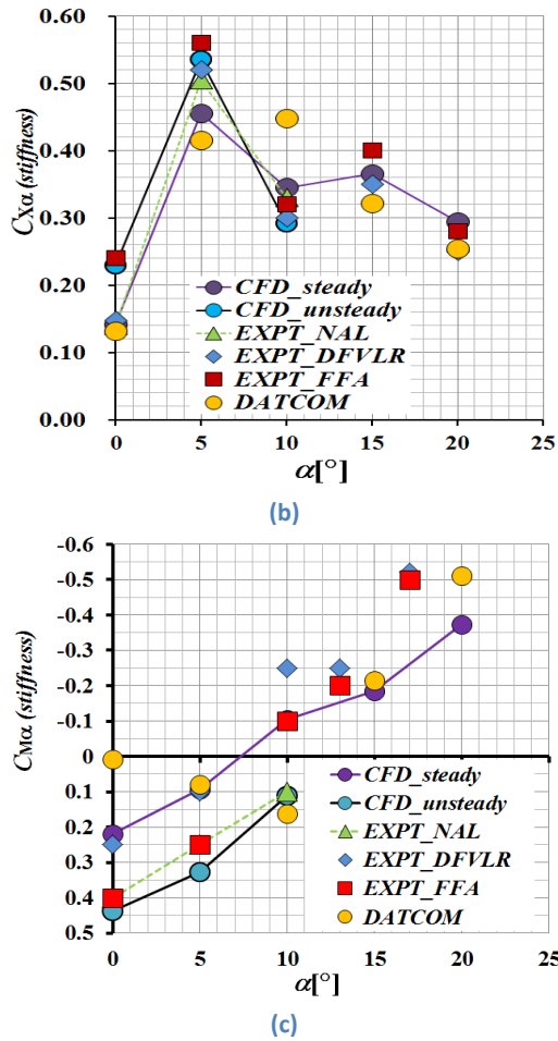
Figure 6. Comparison of stiffness derivatives among CFD, DATCOM and experiment results. (a) C_{Z\alpha} versus angle of attack, (b) C_{X\alpha} versus angle of attack, and (c) C_{M\alpha} versus angle of attack.
